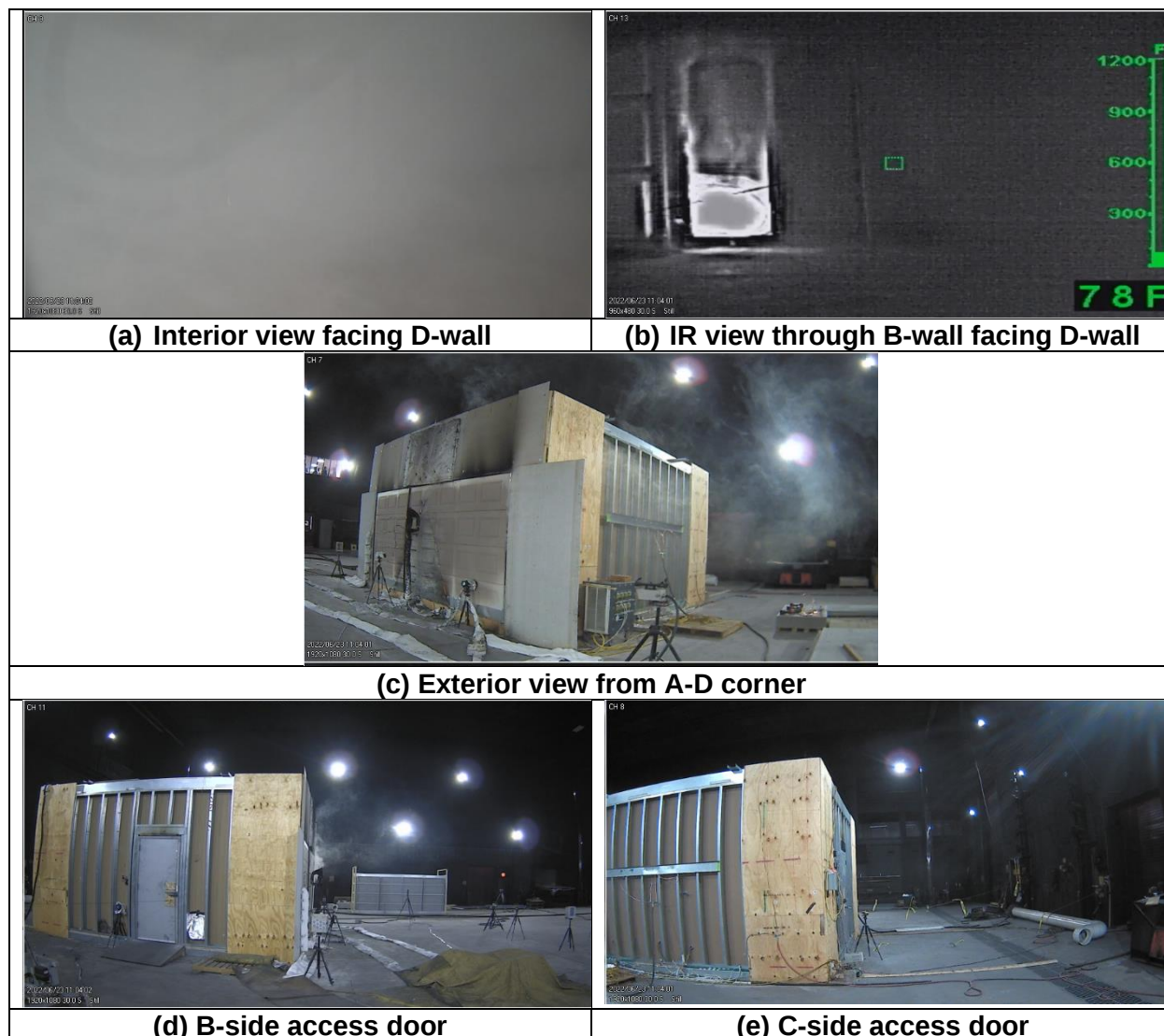
Figure 107 – Exterior view during propagating thermal runaway (30:50, TR + 10:20).
