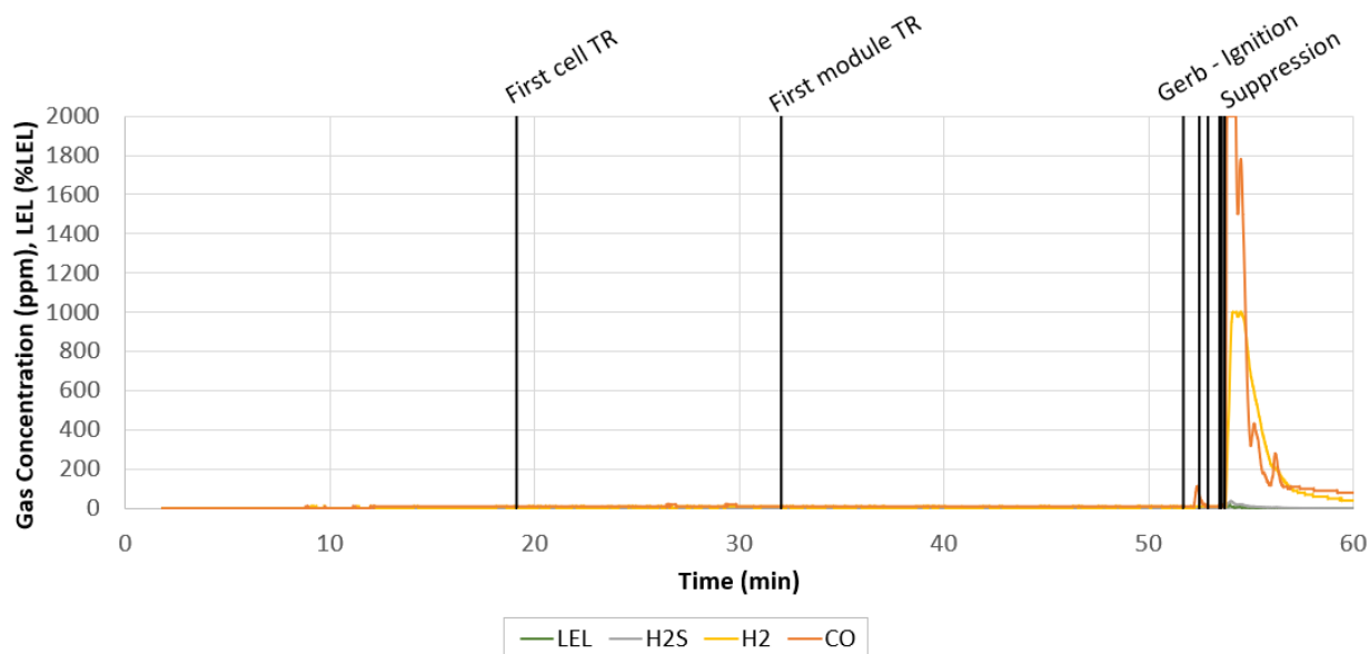
Figure 146 – C-side service door meter measurements during Test 3.
