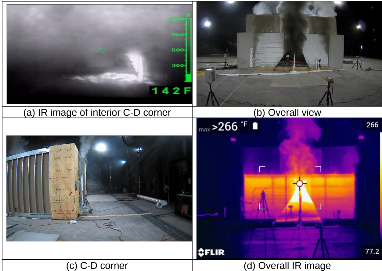
Figure 71 – Images from 1 minute post-ventilation (07:00).
