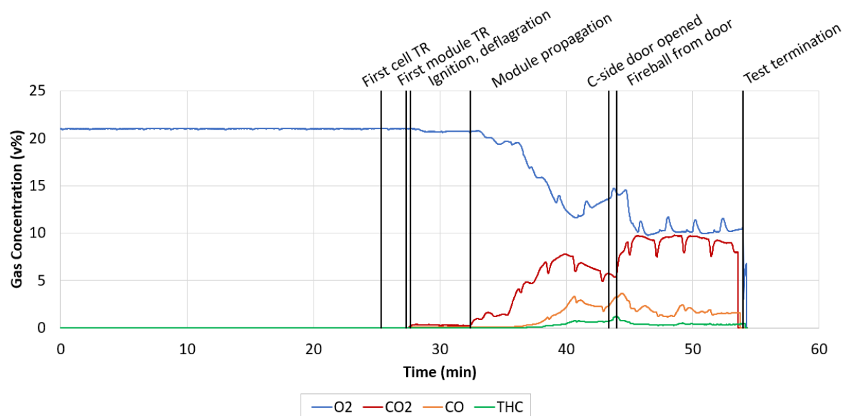
Figure 164 – Interior upper layer gas measurements for Test 4.
