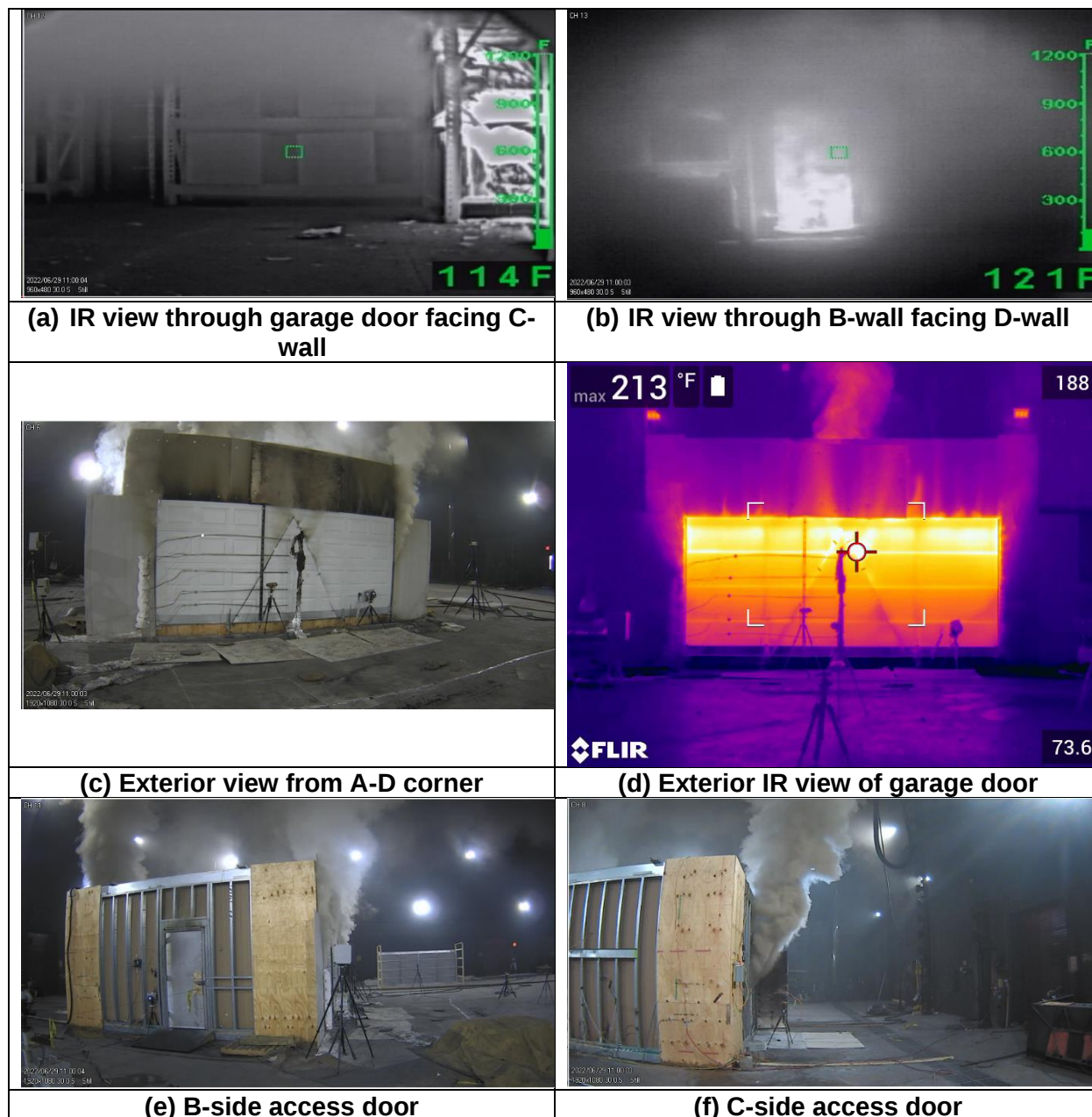
Figure 175 – Conditions prior to backdraft (44:03, TR + 18:42).
