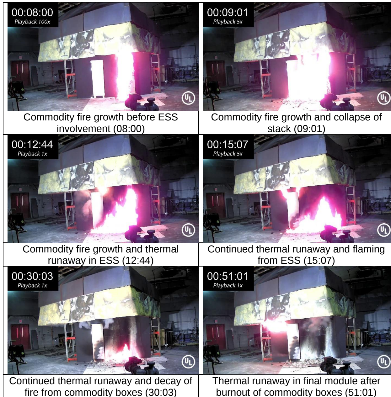
Figure 198 – Images showing test progression in Scenario 2.
