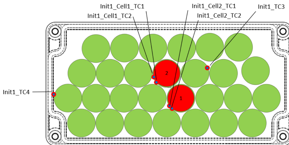
Figure 44 – Initiating module constructed from 18650 cells.
