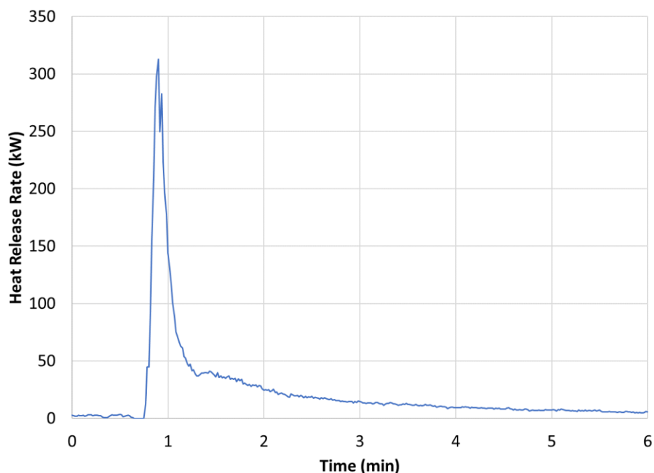
Figure 188 – Module heat release rate.
