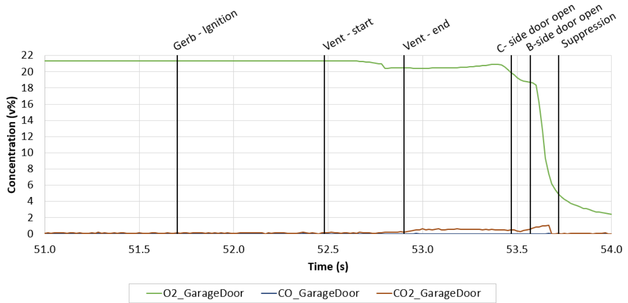
Figure 135 – Exterior gas measurements at the garage door in Test 3.
