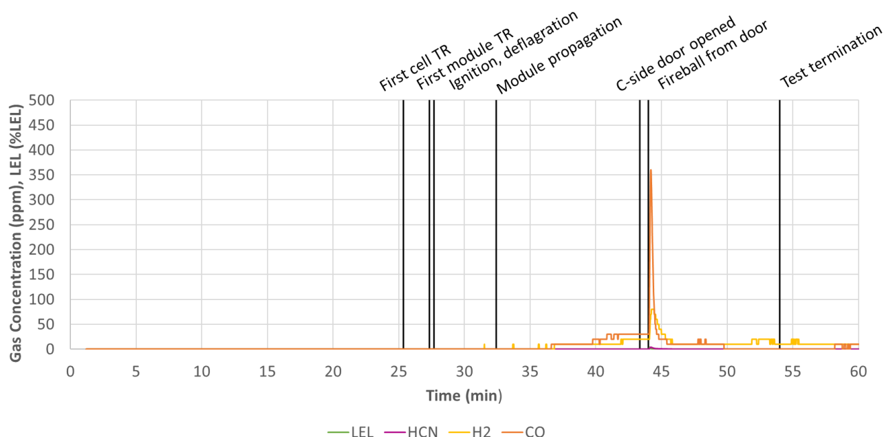
Figure 181 – Measurements at C-side rear door in Test 4.
