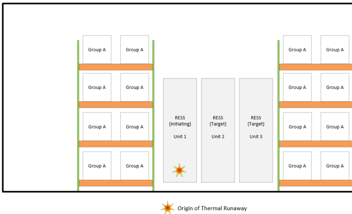
Figure 57 – Location of thermal runaway within Unit 1, shown on D-side wall for Test 2 and Test 4.
