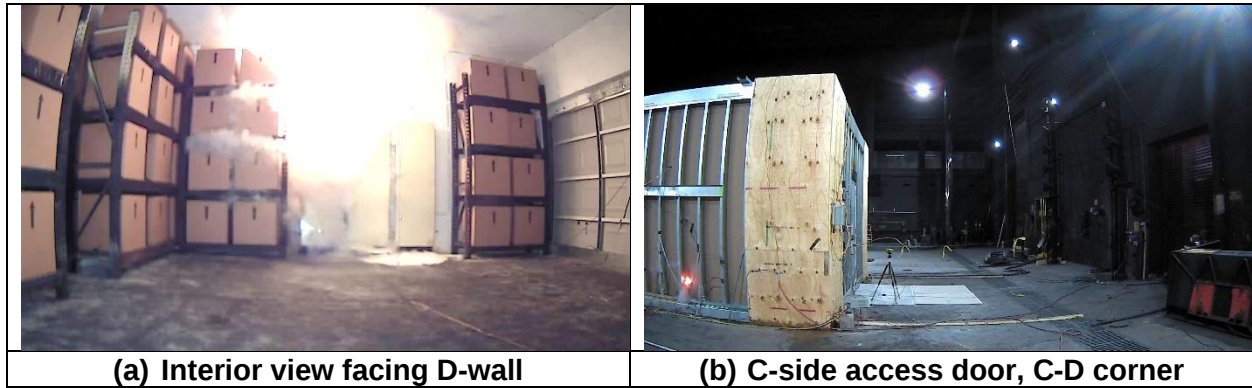
Figure 170 – Flaming observed at penetrations (27:42, TR + 02:21).
