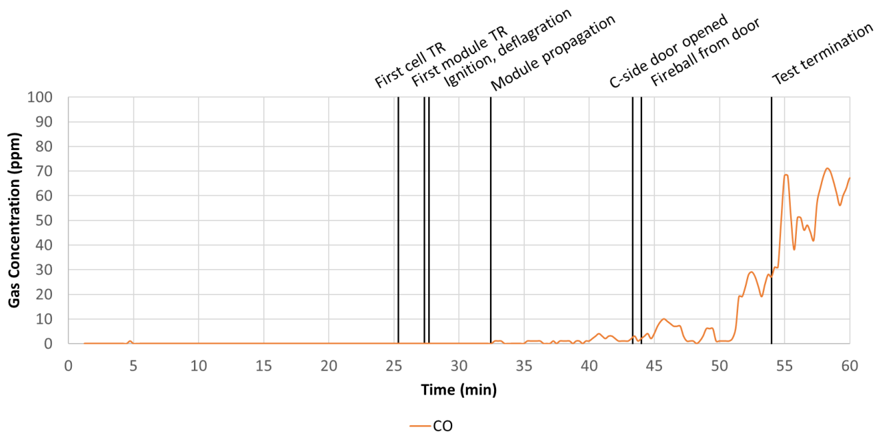
Figure 180 – Measurements at driveway 40 ft location in Test 4.
