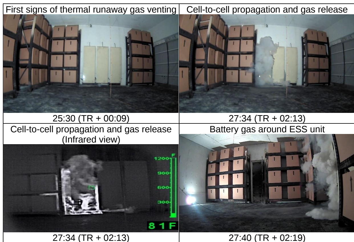
Figure 150 – Test events between 25 and 28 minutes of Test 4.
