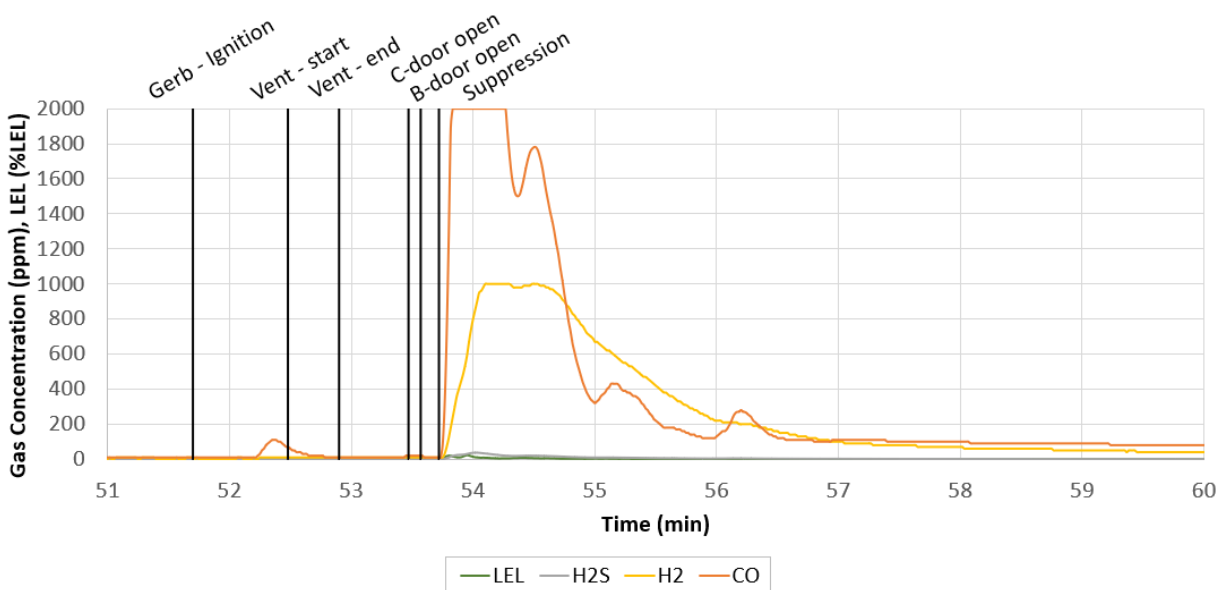
Figure 147 – C-side service door meter measurements during Test 3, for the period between 51 and 60 minutes.
