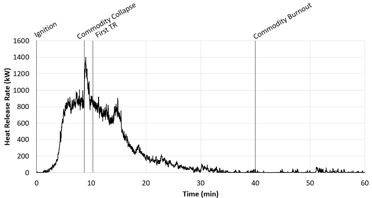
Figure 197 – Heat release rate from the first cell thermal runaway to the end of the test in Scenario 2.
