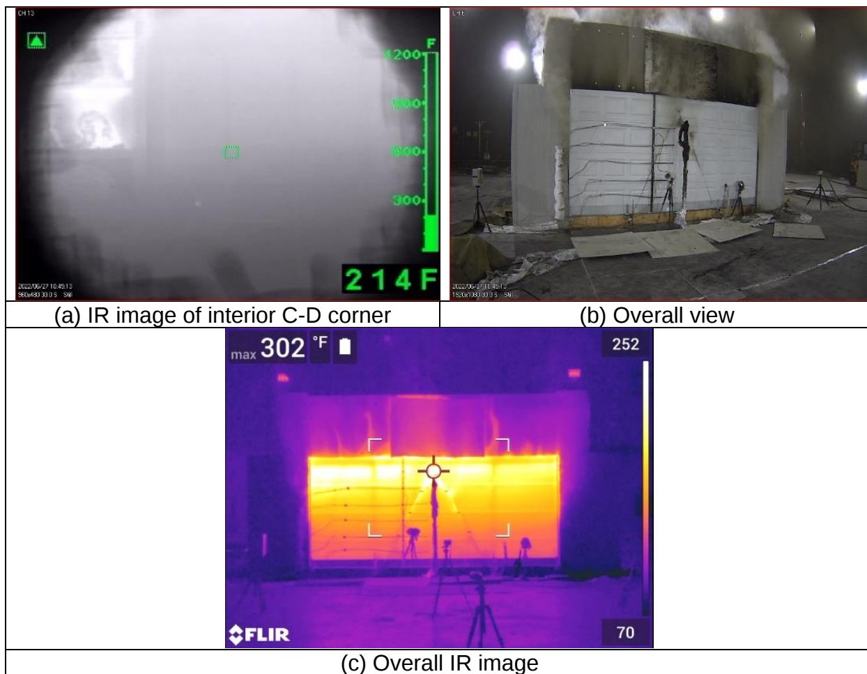
Figure 137 – Images from first module thermal runaway (32:11).
